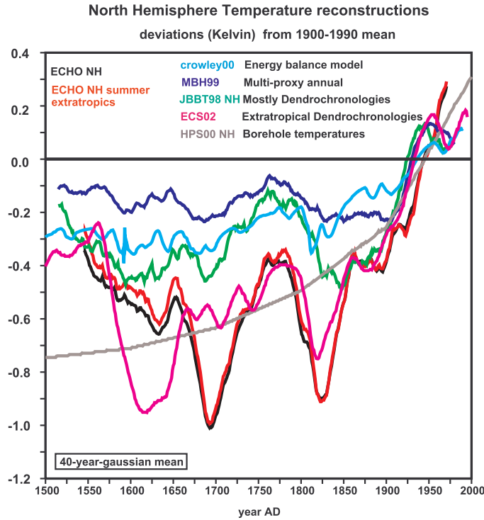
Figure 3: Time series of annual Northern Hemisphere and summer northern extratropics mean temperature anomalies ( deviations from 1900-1990 mean) simulated by the climate model ECHO-G, compared to a simulation with an energy balance model (Crowley, 2000), and with reconstructions of Northern Hemisphere mean temperature based on a multiproxy dataset (MBH99), only dendrochronological data (ECS02), various normalized paleo-data of various types records (JBBT98), and on borehole measurements (HPS00). Time series have been smoothed to represent frequencies lower than 40 years. Note that the individual reconstructions have not been rescaled to represent a common season.
